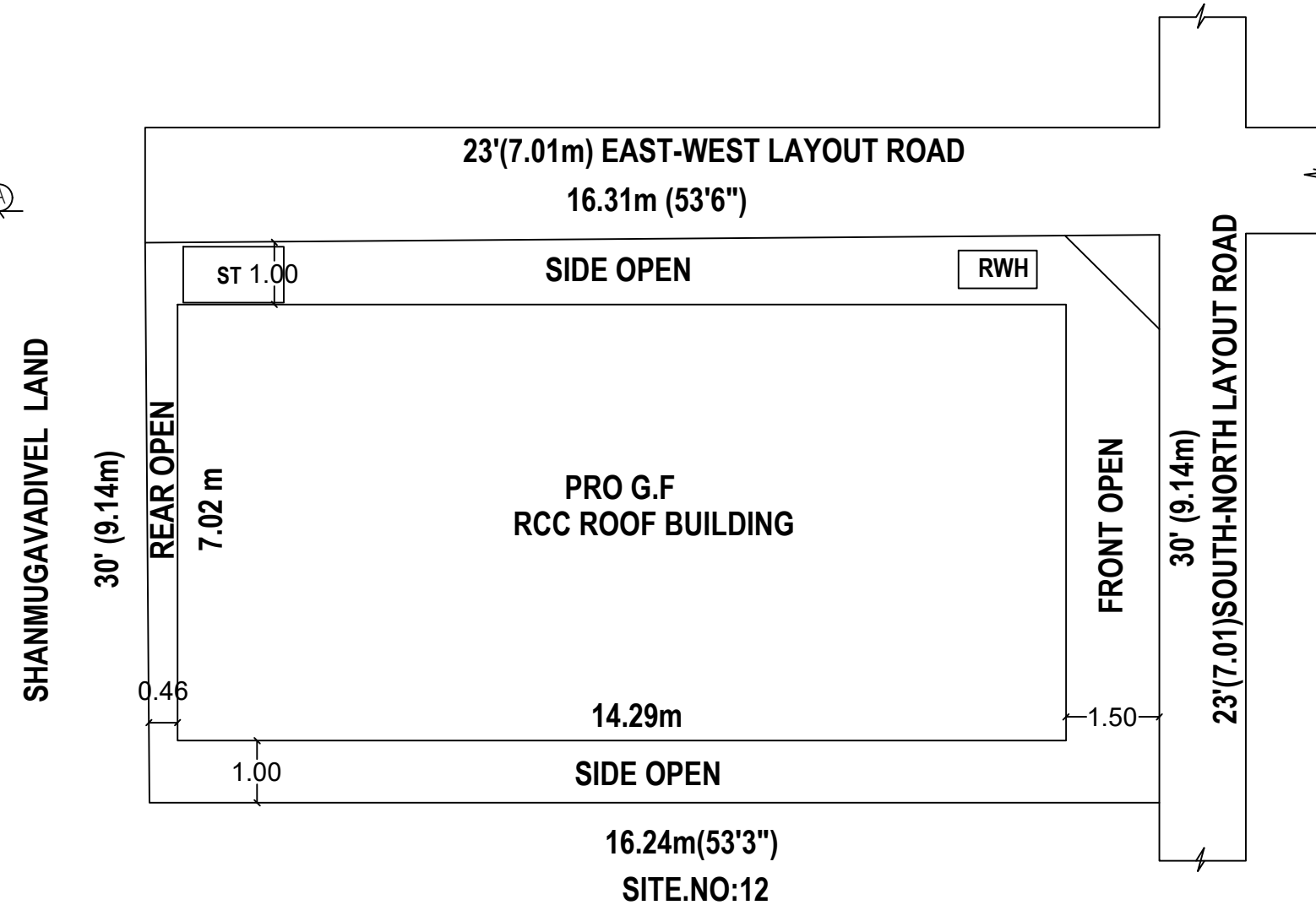
SITE PLAN
