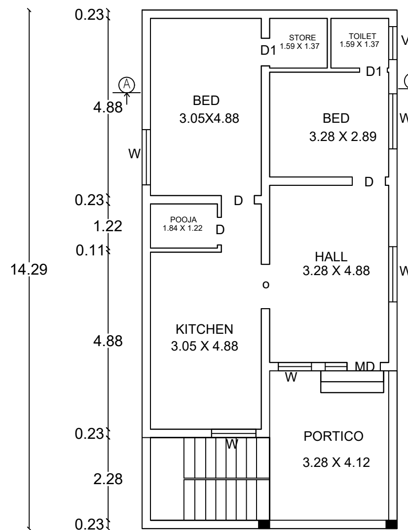
LOOR PLAN
