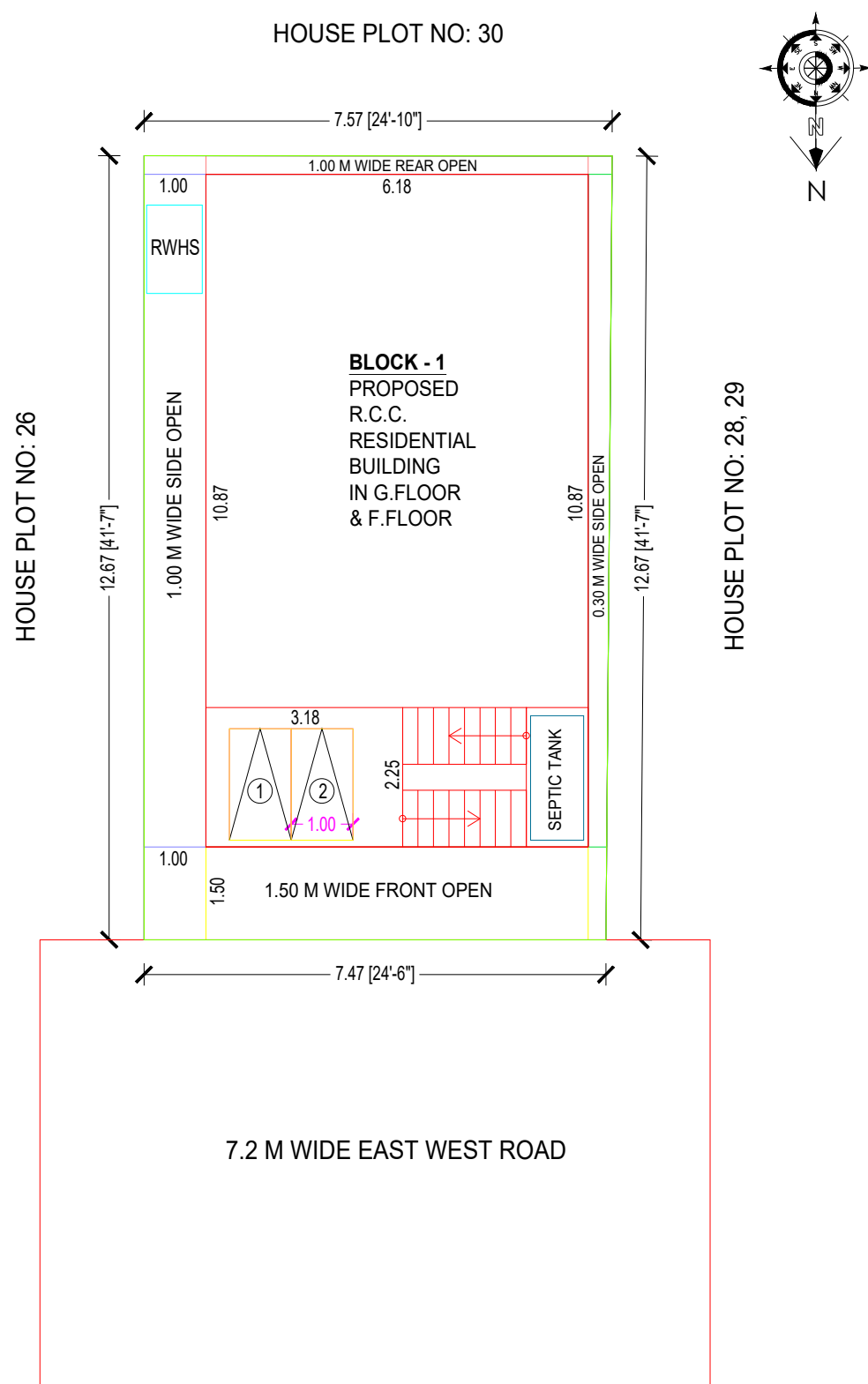
SITE PLAN
