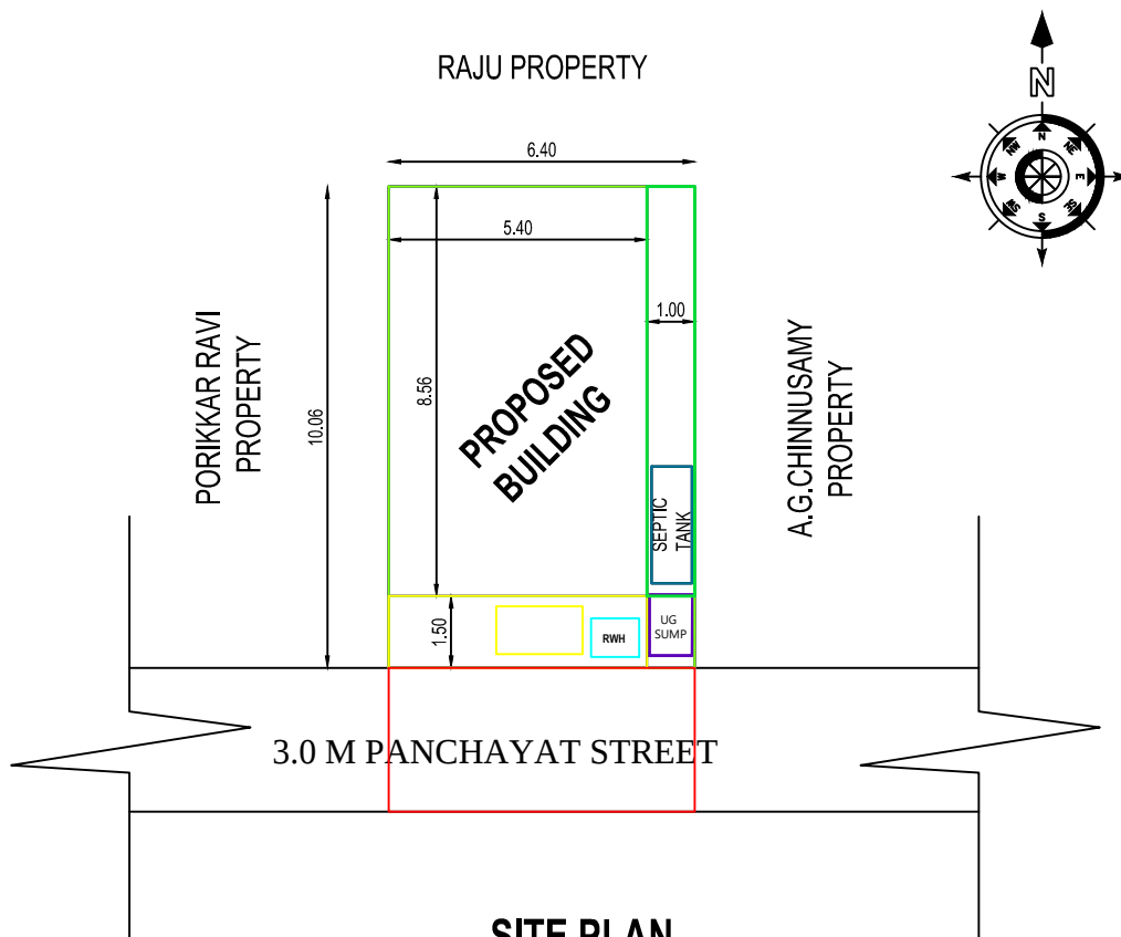
SITE PLAN (Scale : 1:100) ALL DIMENSIONS ARE IN FEET & METRE
