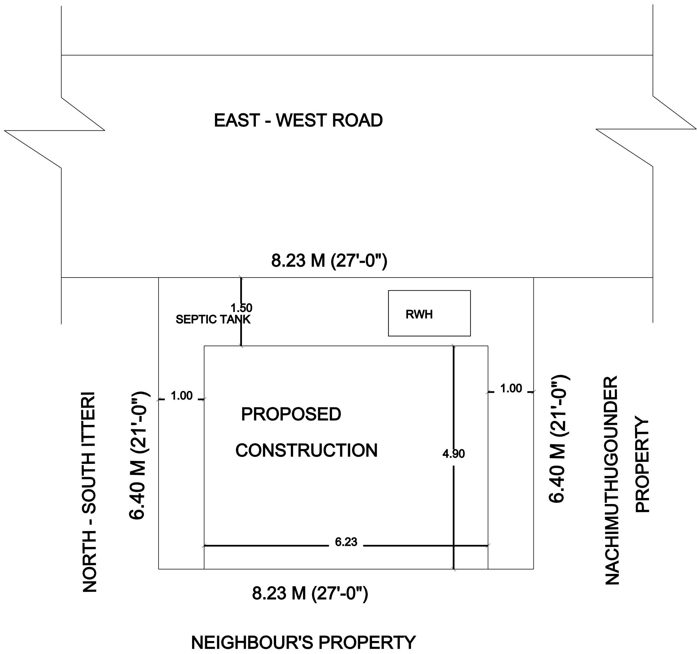
SITE PLAN
