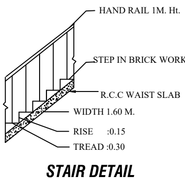
STAIR DETAIL
