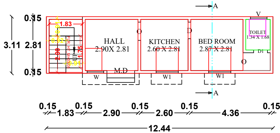
GROUND FLOOR PLAN ( East Facing )
