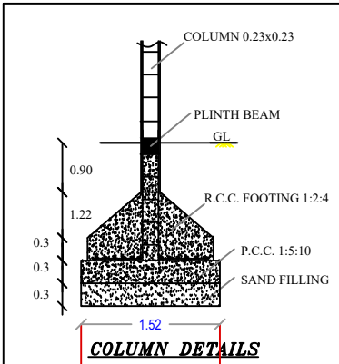
COLUMN DETAILS
