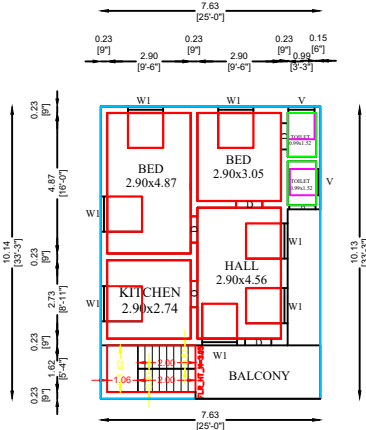
FIRST FLOOR PLAN (PROPOSED BUILDING)
