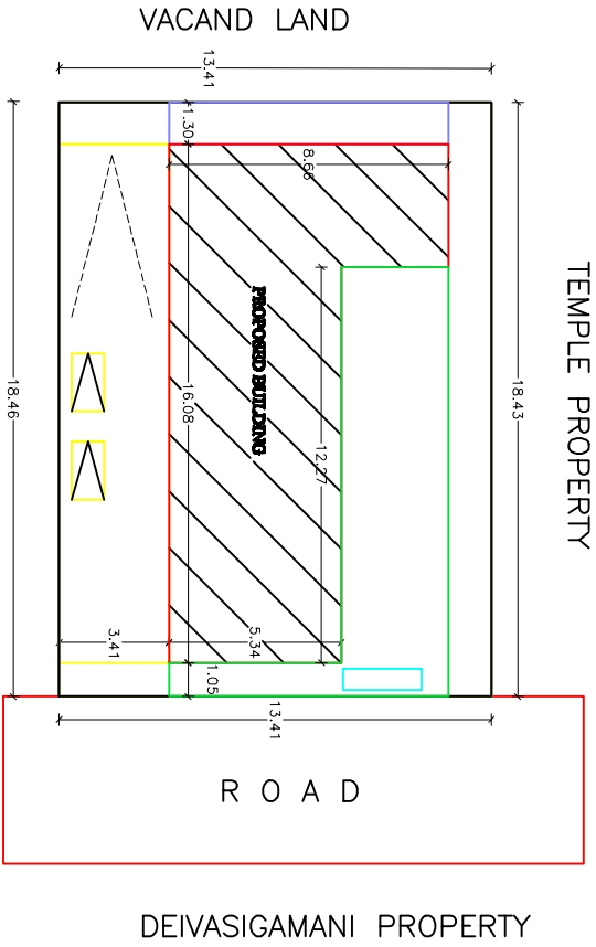
DETAILED PLAN: SCALE 1:100
