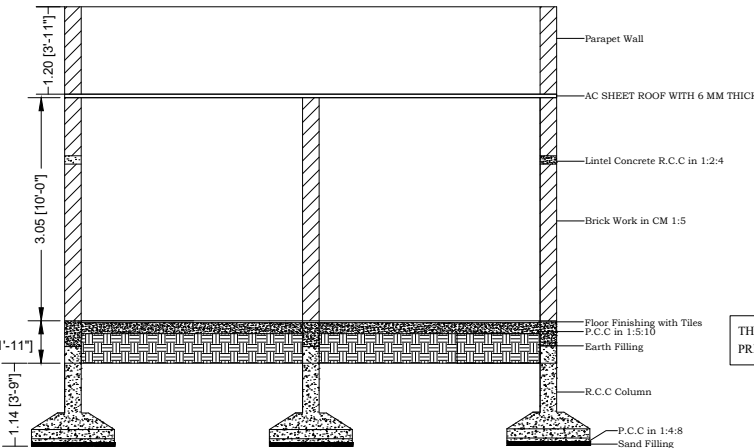
SECTION X-X
