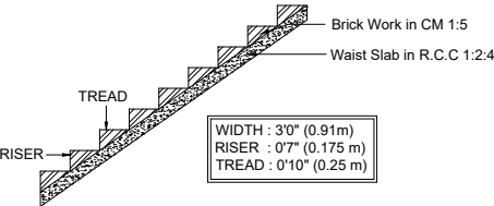
STAIRCASE DETAILS
