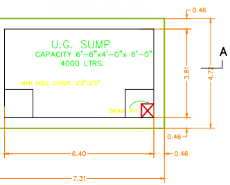
PLAN OF U.G. SUMP SCALE 1"=4'0"
