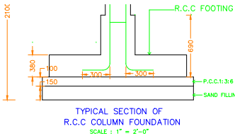
TYPICAL SECTION OF R.C.C COLUMN FOUNDATION SCALE : 1" = 2'-0"
