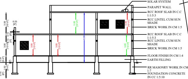
SECTION "AA","BB"
