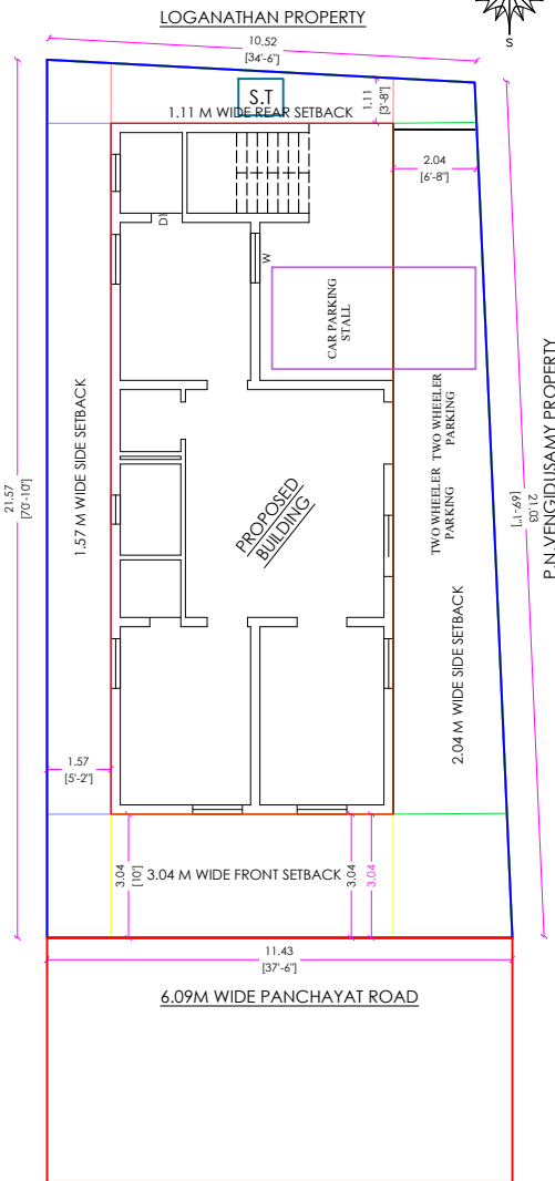
DETAILED SITE PLAN SCALE 1:100
