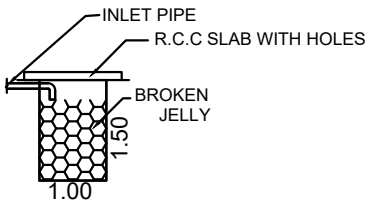
RAIN WATER HARVESTING FILTER BED
