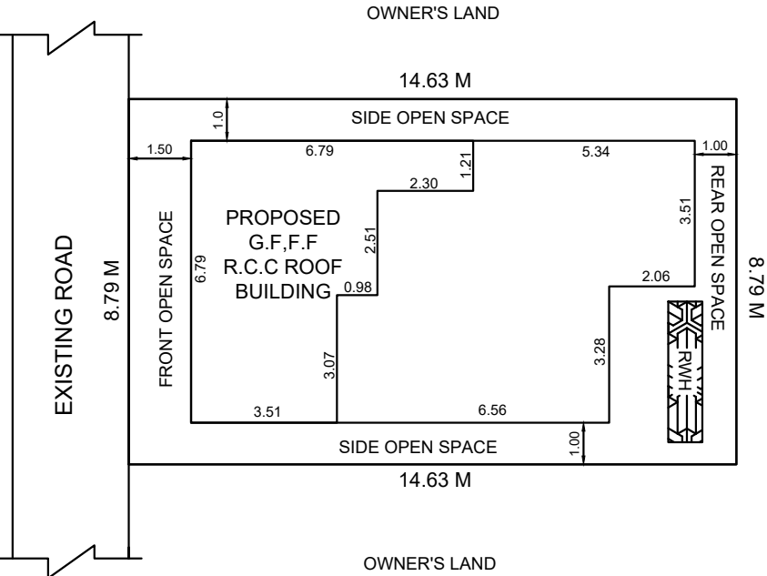
SITE PLAN SCALE 1CM:1M
