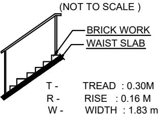
STAIR DETAILS :-
