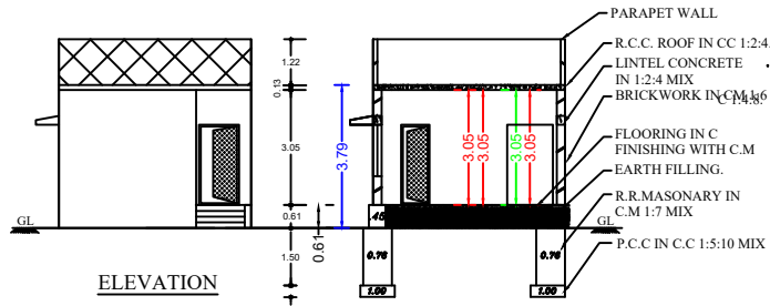
SECTION HK'
