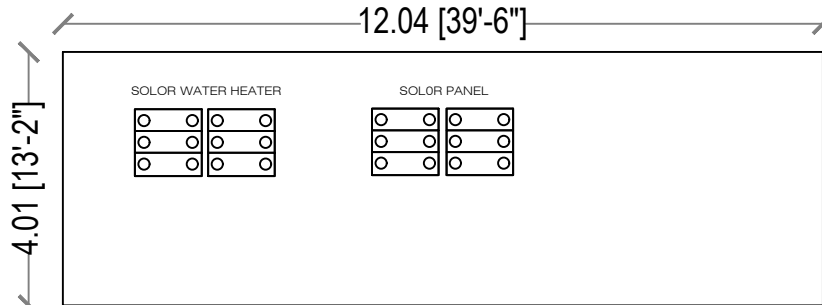
TERRACE PLAN
