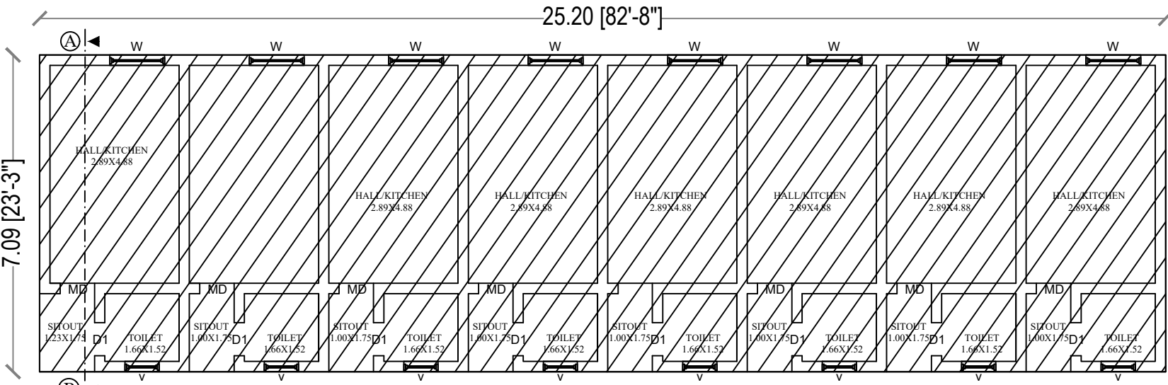
EXISTING RESIDENTIAL GROUND FLOOR AC SHEET PLAN DOOR NO: 223,224,225,226,227,228,229,230 ASSESMENT NO:1499,1500,1501,1502,1503,1504,1505,1507
