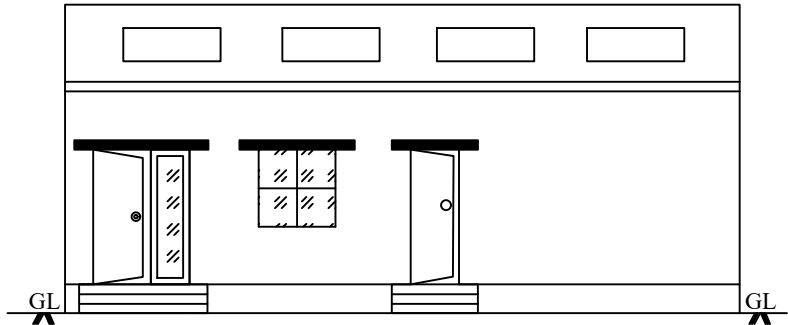
FRONT ELEVATION
