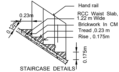
STAIRCASE DETAILS
