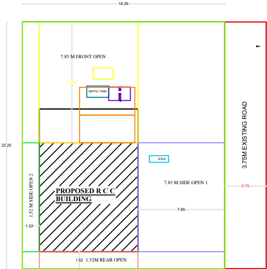
SITE PLAN
