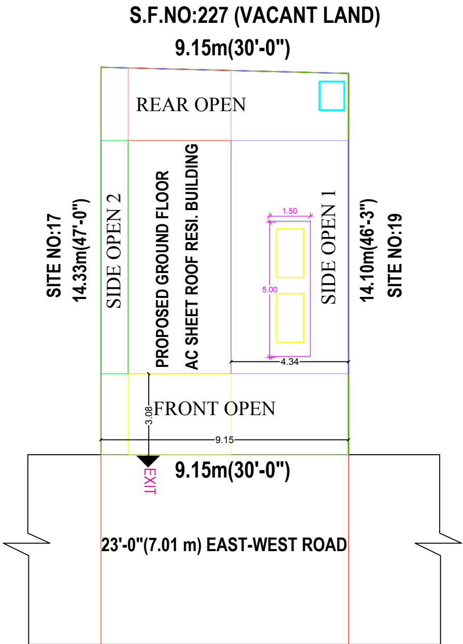
SITE PLAN
