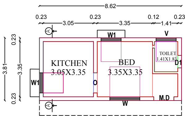
PROPOSED.GF.PLAN
