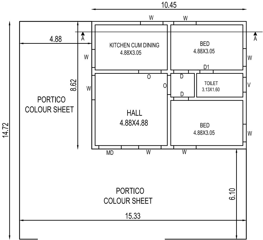
FLOOR PLAN @ 1:100)
