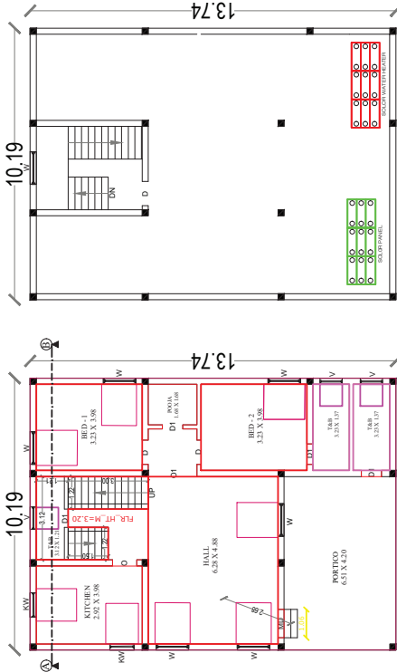
GROUND FLOOR RCC PLAN
