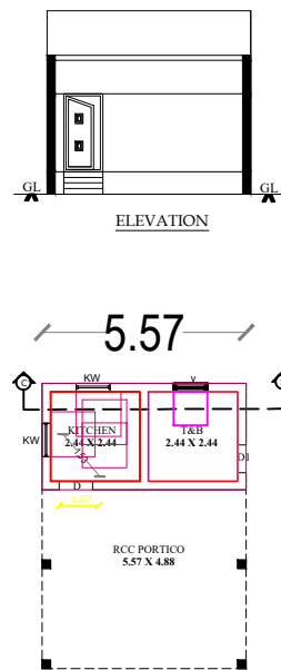
GROUND FLOOR RCC PLAN-II
