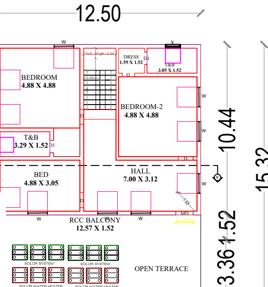
FIRST FLOOR RCC PLAN-I
