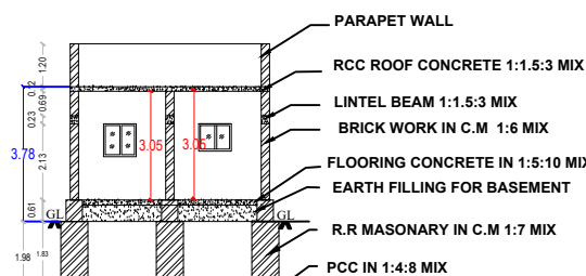
SECTION ON "CD"
