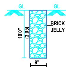
PERCULATION PIT
