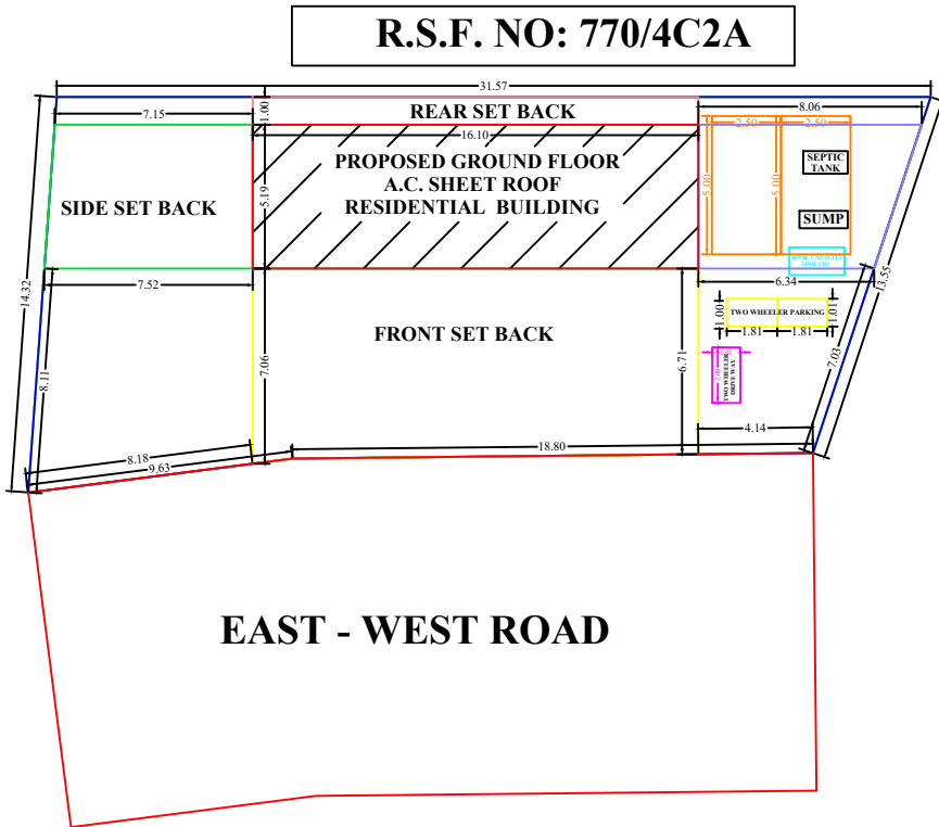
SITE PLAN
