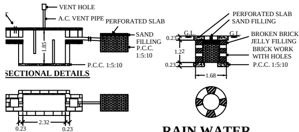
SECTIONAL DETAILS
