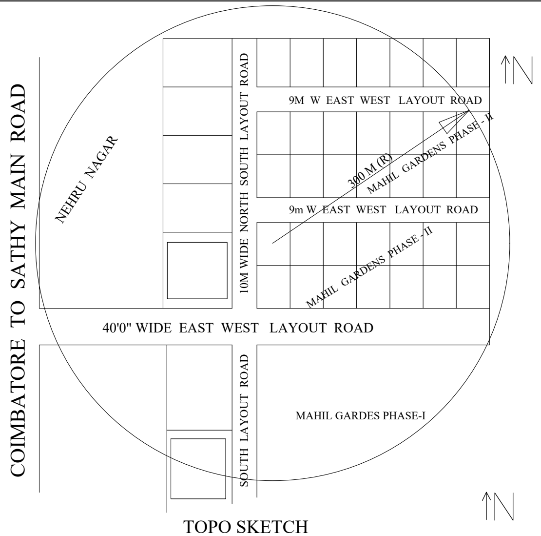
TOPO SKETCH
