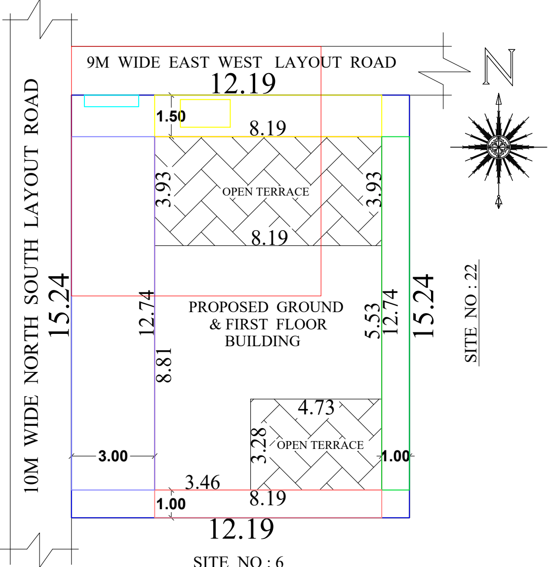
SITE PLAN
