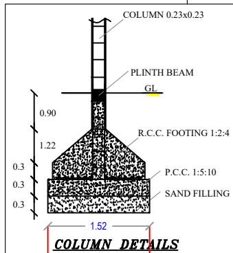
COLUMN DETAILS
