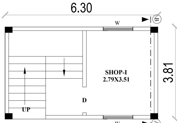
FIRST FLOOR RCC PLAN
