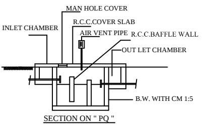
SECTION ON "PQ"
