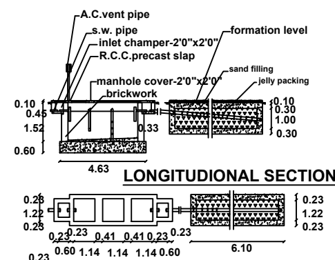
SEPTIC TANK DISPERSION TRENCH
