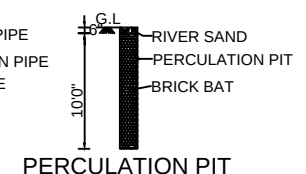
PERCULATION PIT
