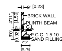
SECTION - CC
