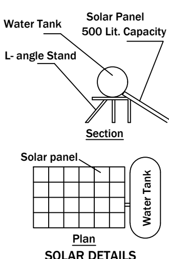
SOLAR DETAILS
