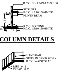
STAIR DETAILS
