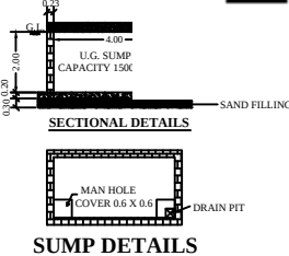
SUMP DETAILS
