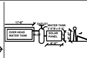
SOLAR WATER HEATER DETAILS
