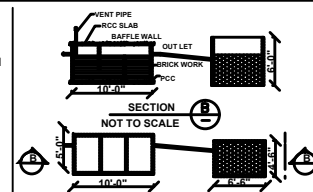
SEPTIC TANK WITH DISPERSION TRENCH
