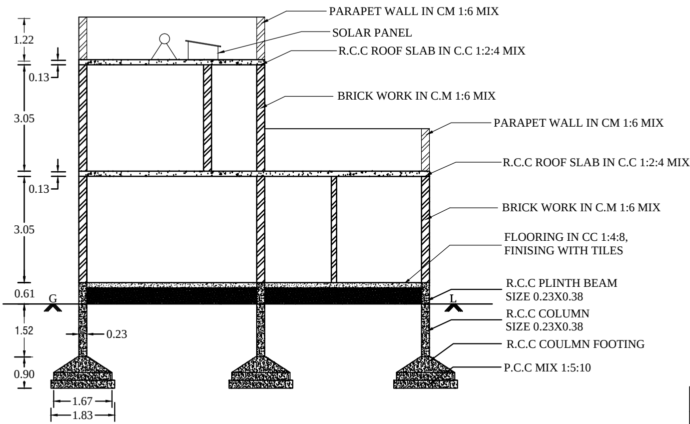
SECTION "A-B"
