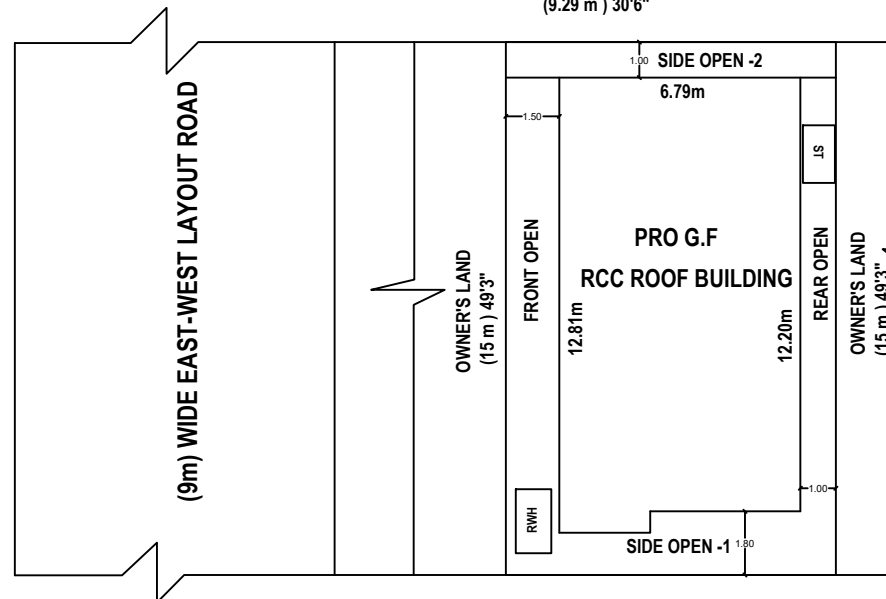
SITE PLAN
