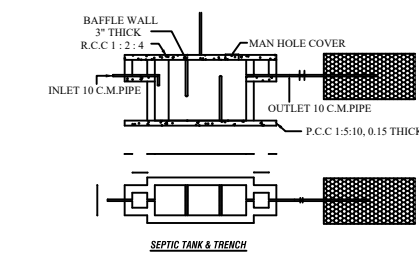
SEPTIC TANK & FRENCH
