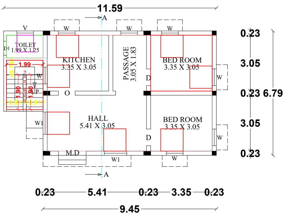
GROUND FLOOR PLAN ( North Facing )
