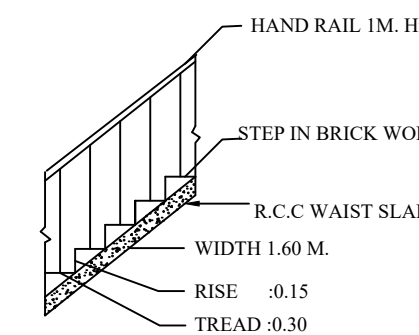
STAIR DETAIL
