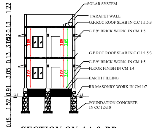
SECTION ON AA & BB
