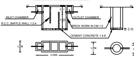
DETAILS OF SEPTIC TANK & SOAK PIT.
