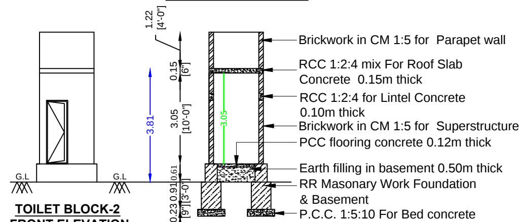
SECTION ON "CD"
