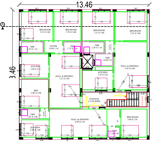
TYPICAL FIRST & SECOND FLOOR RCC PLAN
