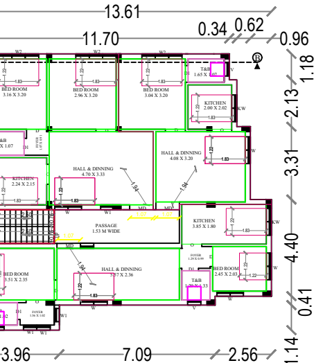
TYPICAL FIRST & SECOND FLOOR RCC PLAN
