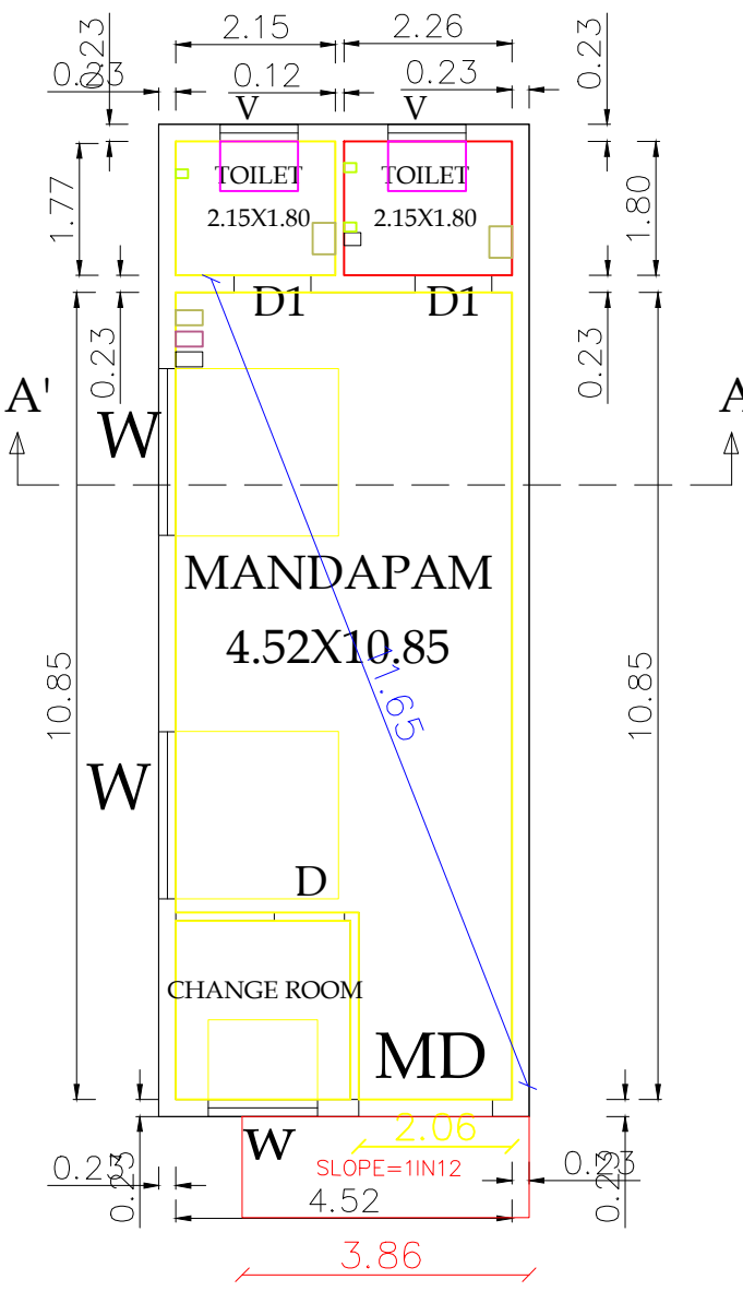
GROUND FLOOR
