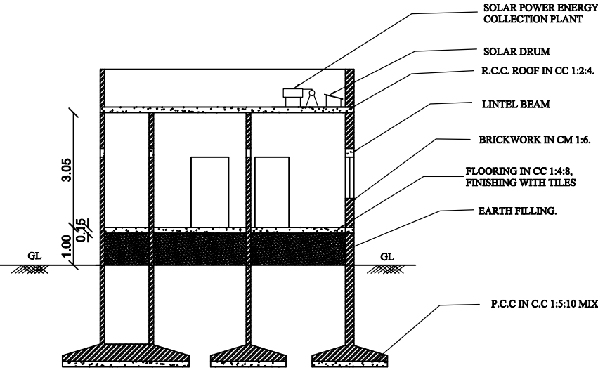
SECTION ON AB & CD
