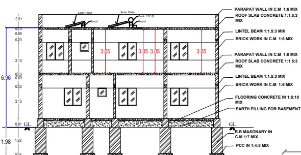
SECTION-A-B
