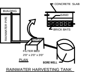
RAINWATER HARVESTING TANK
