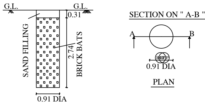
RAINWATER COLLECTION PIT PERCUATION AND DETAILED PLAN
