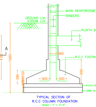
R.C.C COLUMN FOUNDATION SCALE : 1" = 2'-0"
