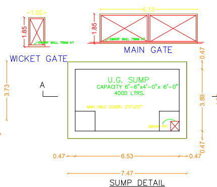
SUMP DETAIL
