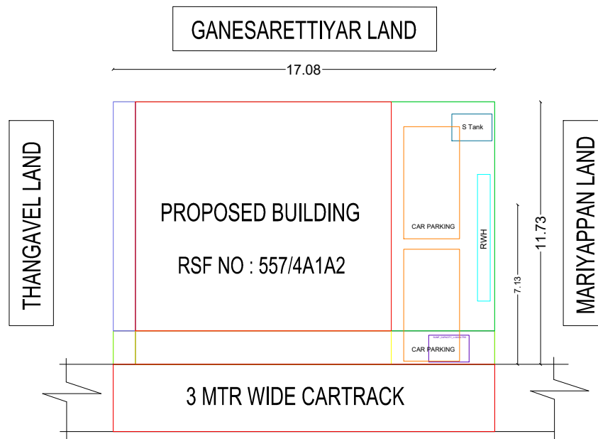
SITE PLAN
