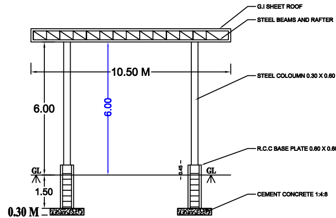
CROSS SECTION
