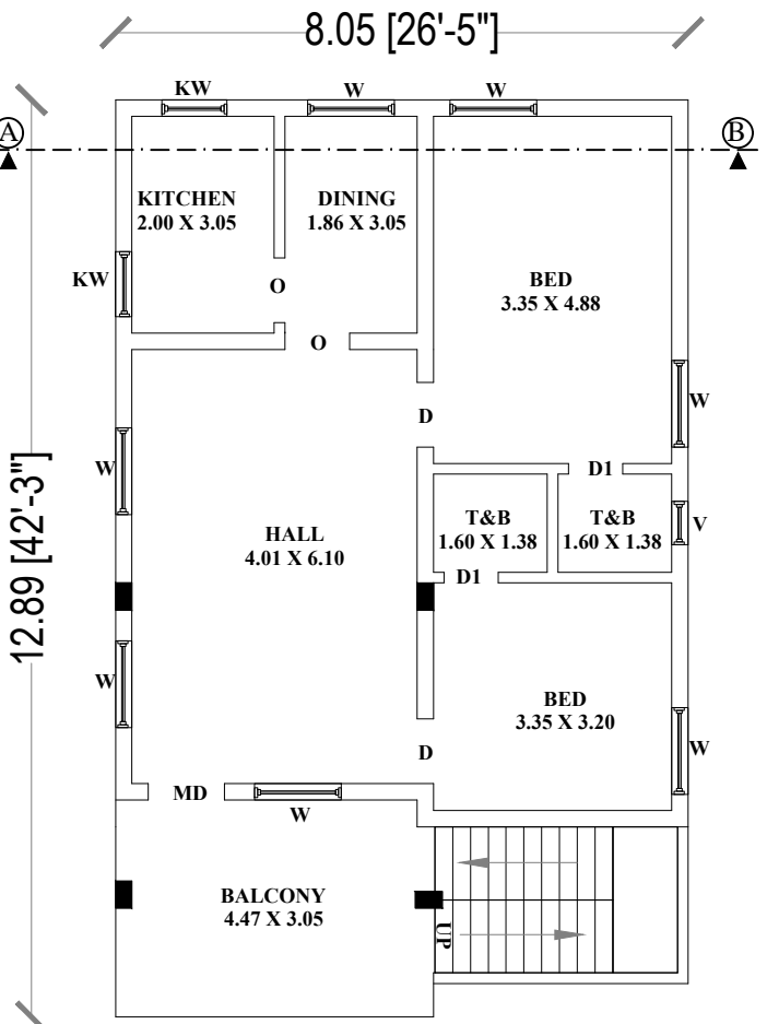
FIRST FLOOR RCC PLAN
