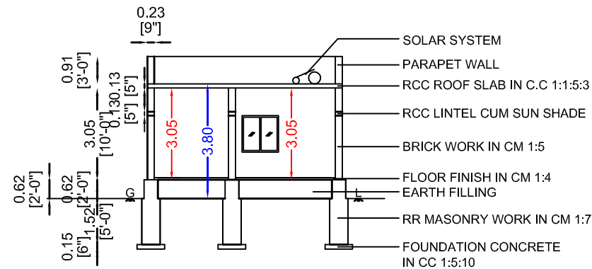
SECTION "AB"
