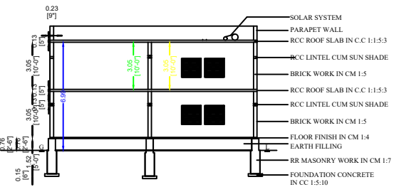
SECTION "AA","BB"
