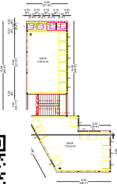
FIRST FLOOR PLAN (COMMERCIAL BUILDING)
