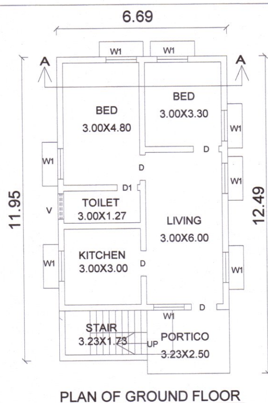
PLAN OF GROUND FLOOR
