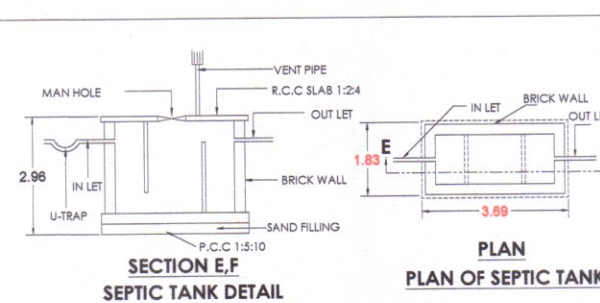
SECTION E-F SEPTIC TANK DETAIL
