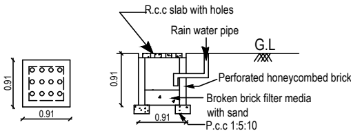
PLAN SECTION RAIN WATER HARVESTING TANK
